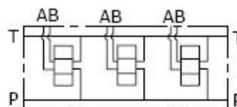
Schema idraulico Hydraulic diagram
