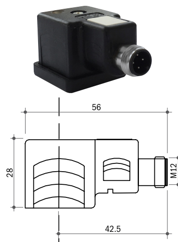
Conector M12
